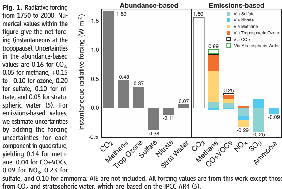
Fig. 1. Radiative forcing from 1750 to 2000. Numerical values within the figure give the net forcing (instantaneous at the tropopause). Uncertainties in the abundance-based values are 0.16 for \text{CO}_2 , 0.05 for methane, +0.15 to -0.10 for ozone, 0.20 for sulfate, 0.10 for nitrate, and 0.05 for stratospheric water (5). For emissions-based values, we estimate uncertainties by adding the forcing uncertainties for each component in quadrature, yielding 0.14 for methane, 0.04 for \text{CO}+\text{VOCs} , 0.09 for \text{NO}_x , 0.23 for sulfate, and 0.10 for ammonia. AIE are not included. All forcing values are from this work except those from \text{CO}_2 and stratospheric water, which are based on the IPCC AR4 (5).
