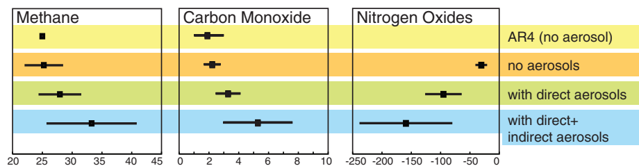
Fig. 2. The 100-year GWPs for methane, CO, and \text{NO}_x (per Tg N) as given in the AR4 and in this study when including no aerosol response, the direct radiative effect of aerosol response, and the direct+indirect radiative effects of aerosol responses. The AR4 did not report uncertainties for methane or CO and gave no mean estimate for \text{NO}_x . The range for the GWP of CO is from the third IPCC assessment and encompasses values reported up through the AR4. Our calculations for the shorter 20-year GWP, including aerosol responses, yield values of 79 and 105 for methane, 11 and 19 for CO, and -335 and -560 for \text{NO}_x , including direct and direct+indirect radiative effects of aerosols in each case. The 100-yr GWPs for \text{SO}_2 (per Tg \text{SO}_2 ) and ammonia would be -22 and -19 , respectively, including direct aerosol radiative effects only, and -76 and -15 adding indirect aerosol radiative effects. GWPs for very short-lived \text{NO}_x , \text{SO}_2 , and ammonia will vary widely by emission location and timing, and hence global values are of limited use.
